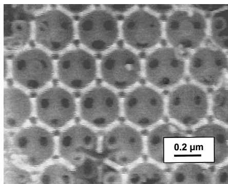
Figure 11. SEM image of a macroporous inorganic material. The walls consist of ~20 nm (\text{VO})_2\text{P}_2\text{O}_7 crystals (modified from ref. [173] ).
